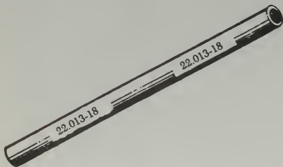
FIGURE 4-86. Wire identification code.
